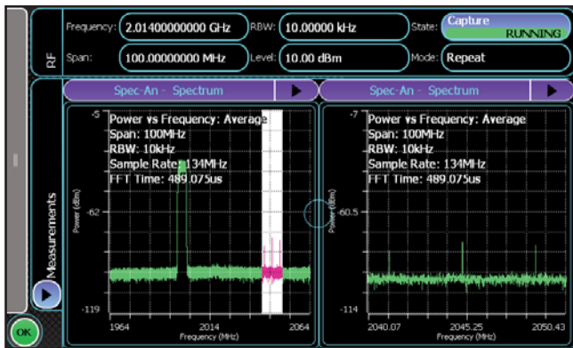
Figure 2. Spectrum Analyzer screenshot of UMTS with spurious signals
