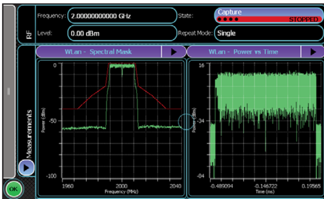
Figure 6. WLAN typical screenshot
