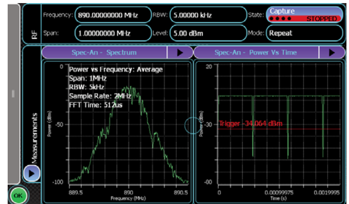
Figure 3. GSM/EDGE screenshot
