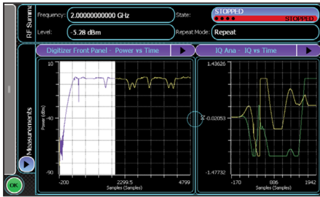
Figure 1. Using drag and drop to analyze a GSM burst
