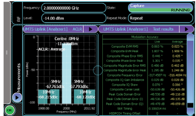
Figure 4. UMTS typical screenshot
